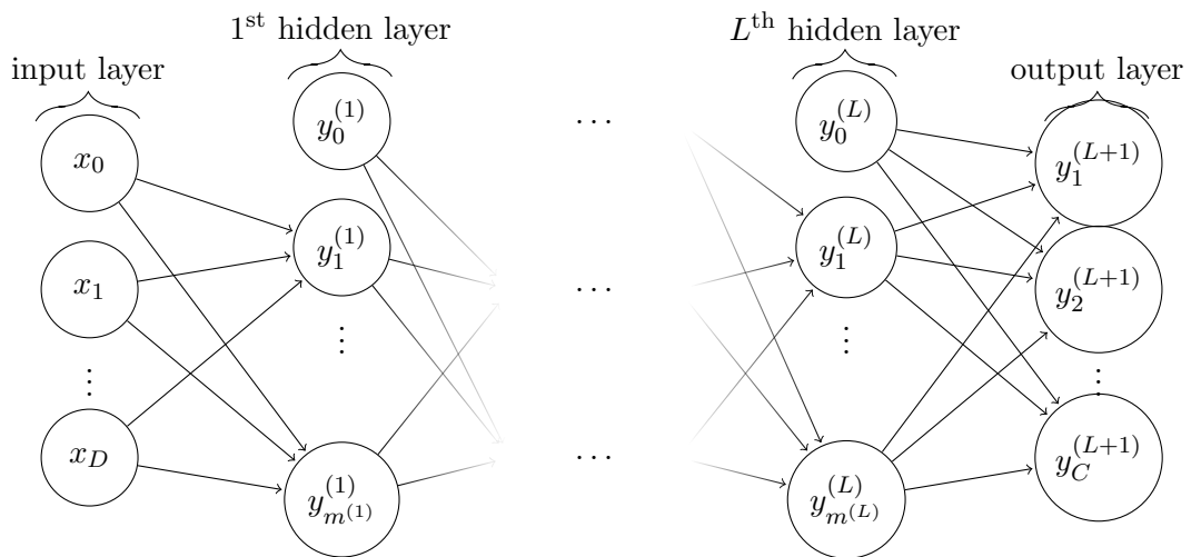
Figure 1: Network graph of a (L + 1) -layer perceptron with D input units and C output units. The l^{\text{th}} hidden layer contains m^{(l)} hidden units.
